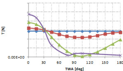
Figure 4: Example of savings on basis of propeller thrust in calm water
