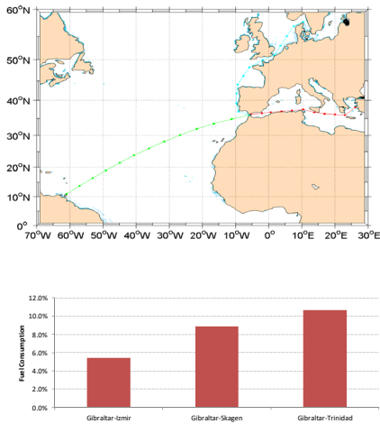
Figure 5: Fuel savings based on hindcast environmental data for specific routes [0]
